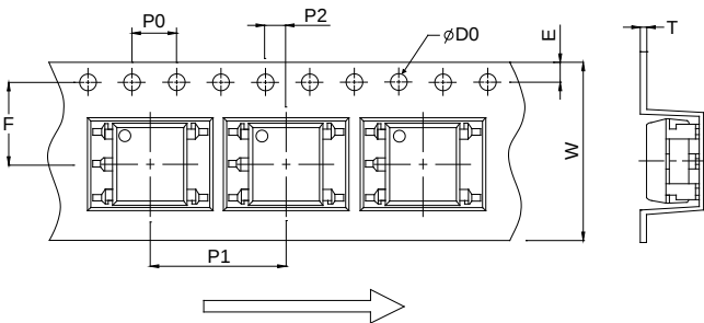
Option SL(T1)
