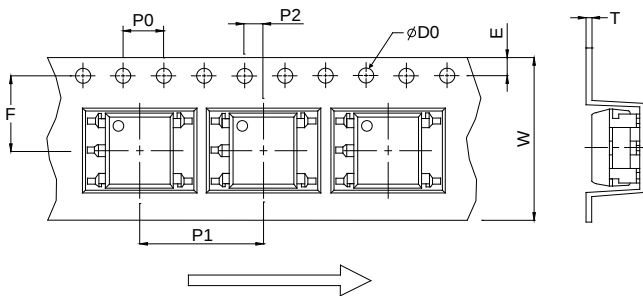
Option S(T1)
